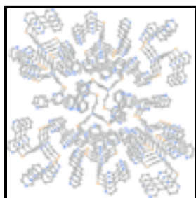
Fig. 2. A section of the three-dimensional supramolecular network of the title compound viewed down the c -axis.
