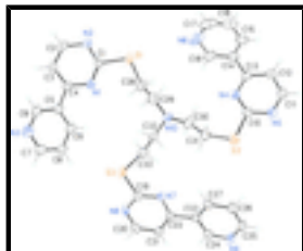
Fig. 1. The molecular structure of the title compound with labelled non-hydrogen atoms. Displacement ellipsoids are drawn at the 20% probability level.
